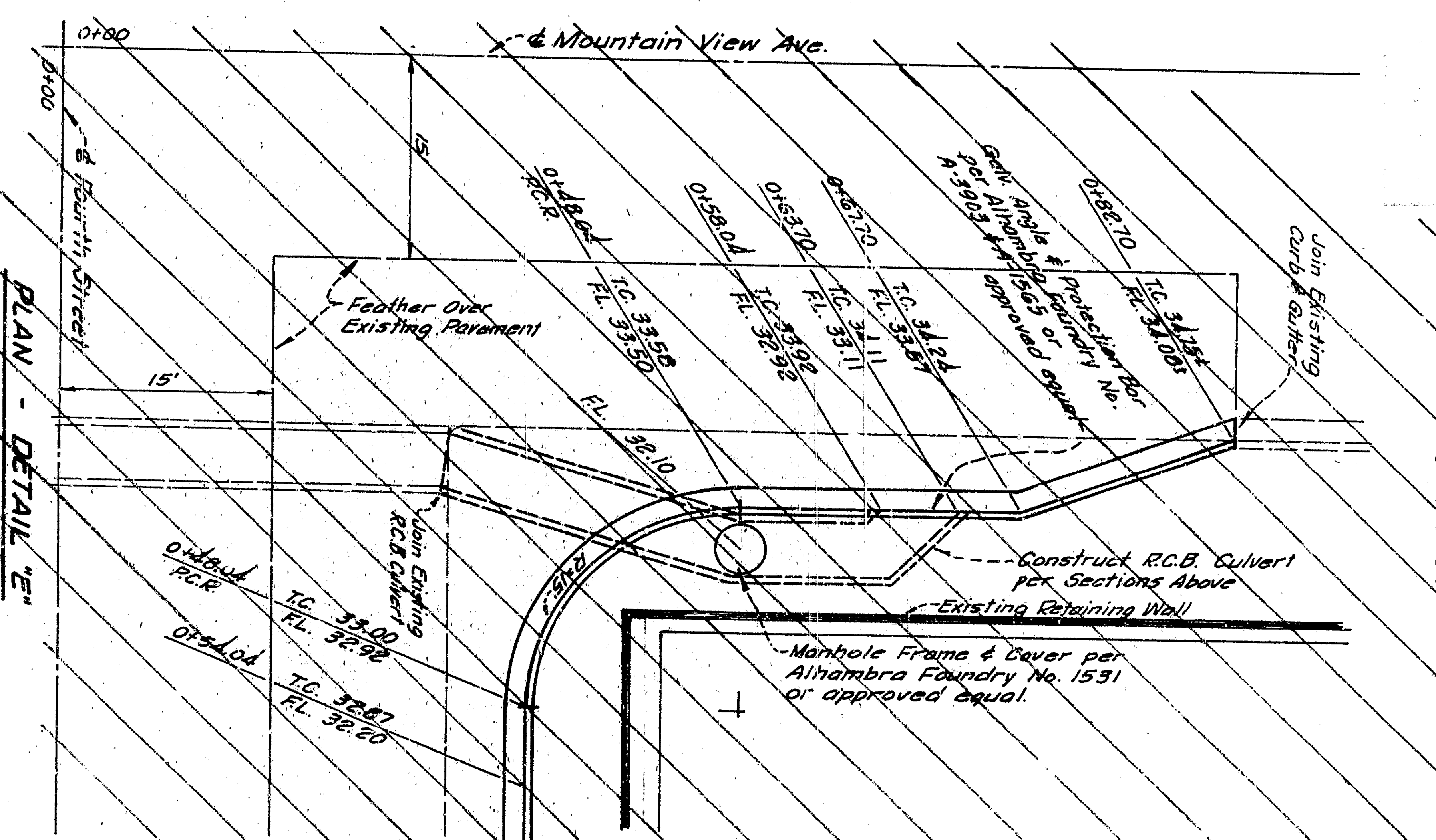
PLAN - DETAIL 'E' Scale: 1"=10'
