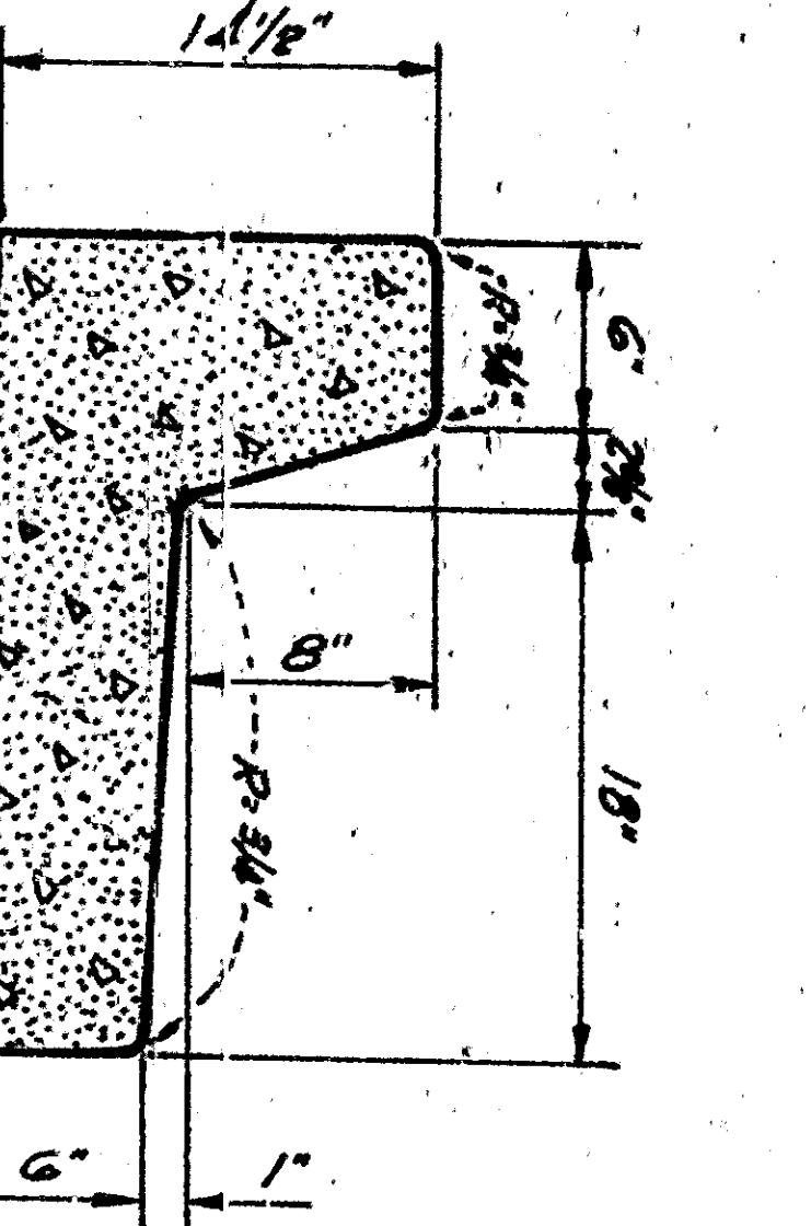
DETAIL 'B' Modified Type 'B' Curb & Gutter No Scale
